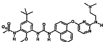
N-[5-tert-Butyl-3-(3-{4-[2-(2-dimethylamino-ethylamino)-pyrimidin-4-yloxy]-naphthalen-1-yl}-ureido)-2-methoxy-phenyl]-methanesulfonamide;
